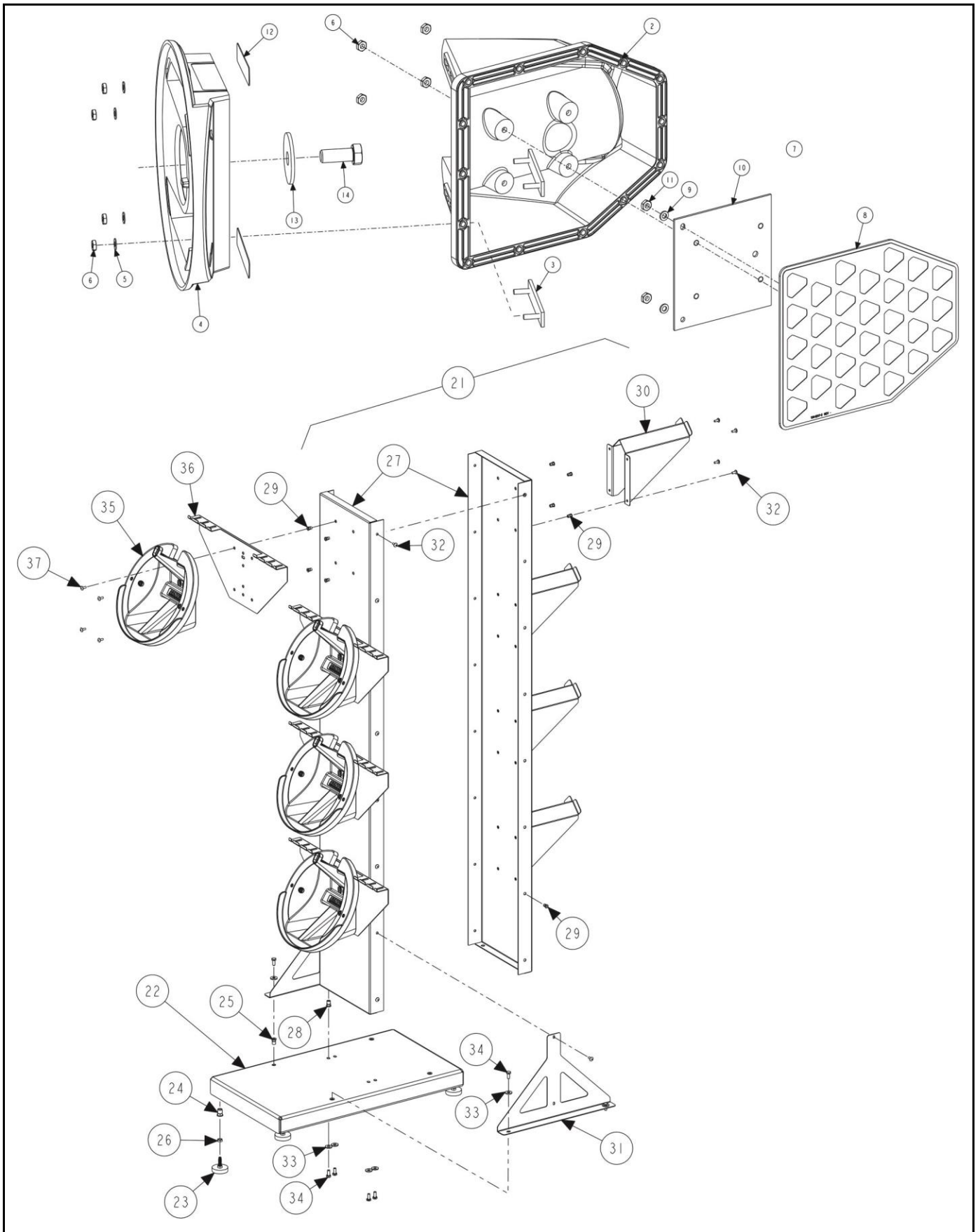
HQ TARGETS AND STORAGE STAND PARTS DRAWING
