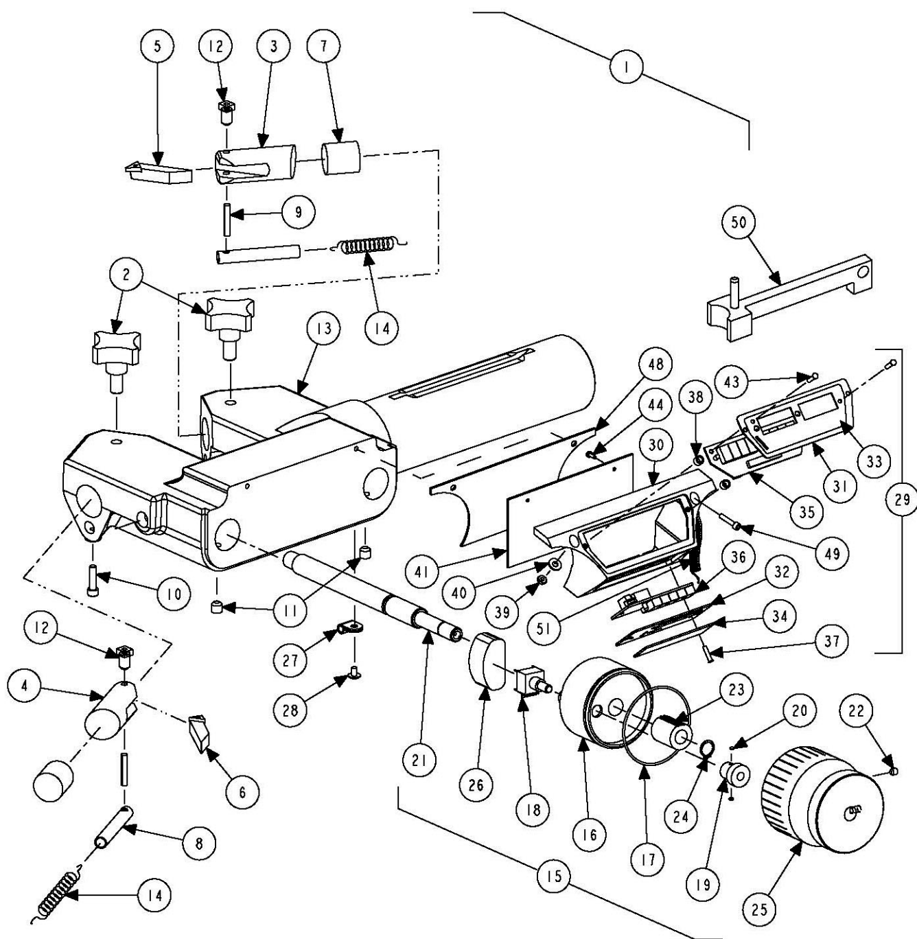
TWIN CUTTER WITH DIGICAL HOUSING 105-389-1 ONLY
