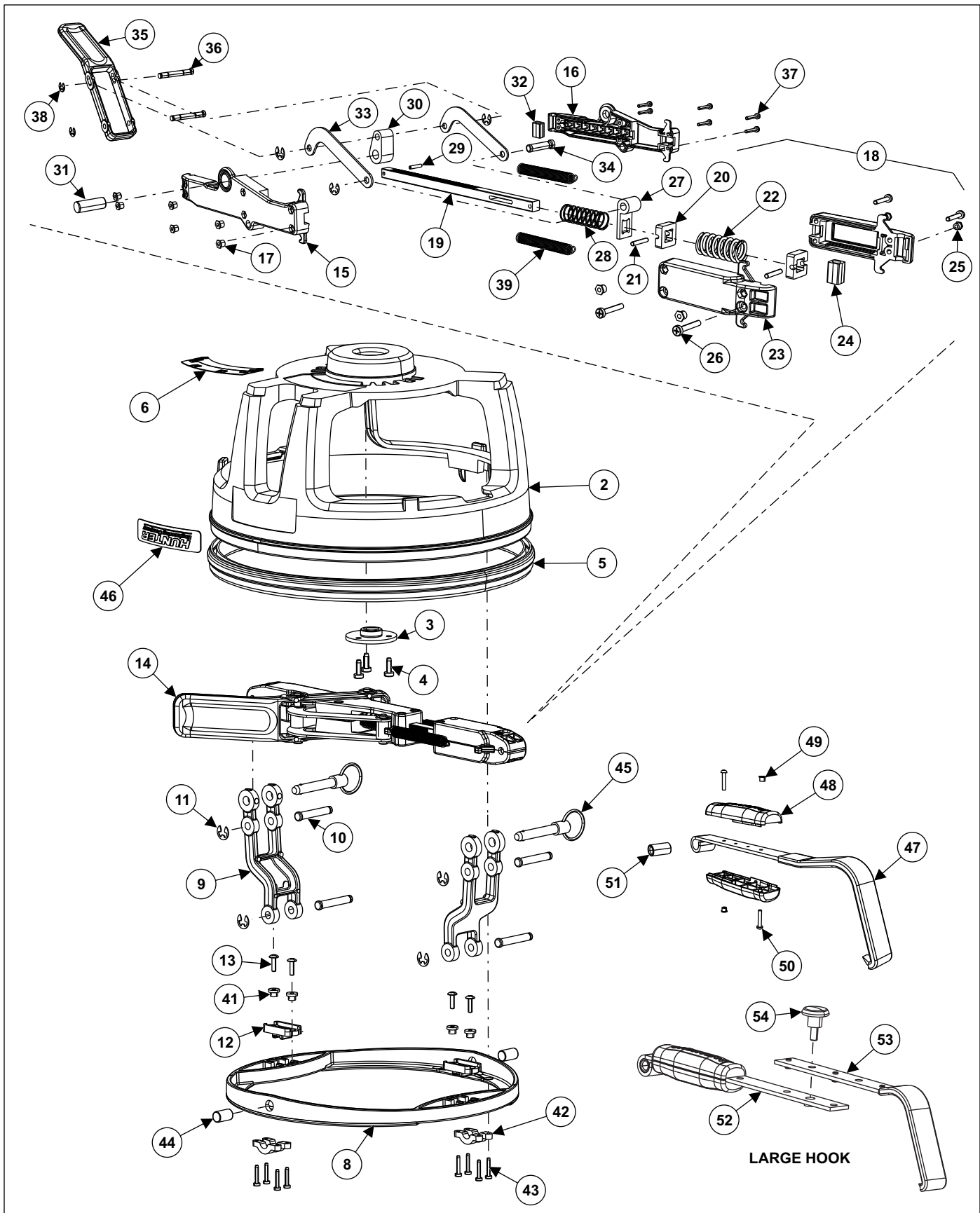
QuickGrip® Adaptor 175-409-1 REFER TO NEXT SHEET FOR PARTS DESCRIPTION LISTING
